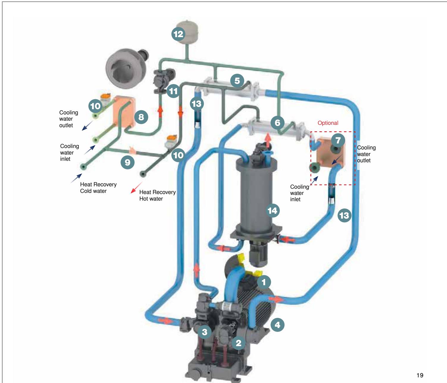
Fig 2: Version with rotation dryer
